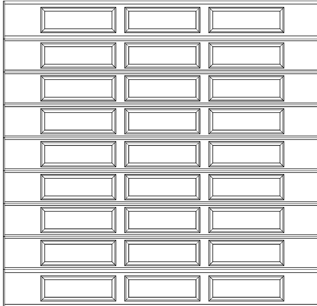
14'6" X 14'0" 8300/8500 ERP DESIGN 8 SECTION/ 3 PANEL SOLID TOP SECTION (7) 18" & (2) 20.8" SECTIONS
