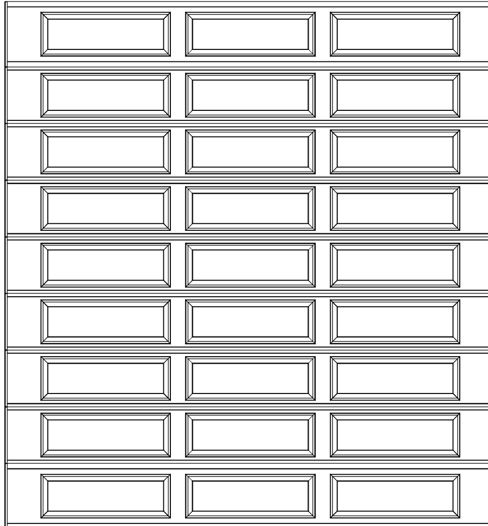
13'0" X 14'0" 8300/8500 ERP DESIGN 8 SECTION/ 3 PANEL SOLID TOP SECTION (7) 18" & (2) 20.8" SECTIONS
