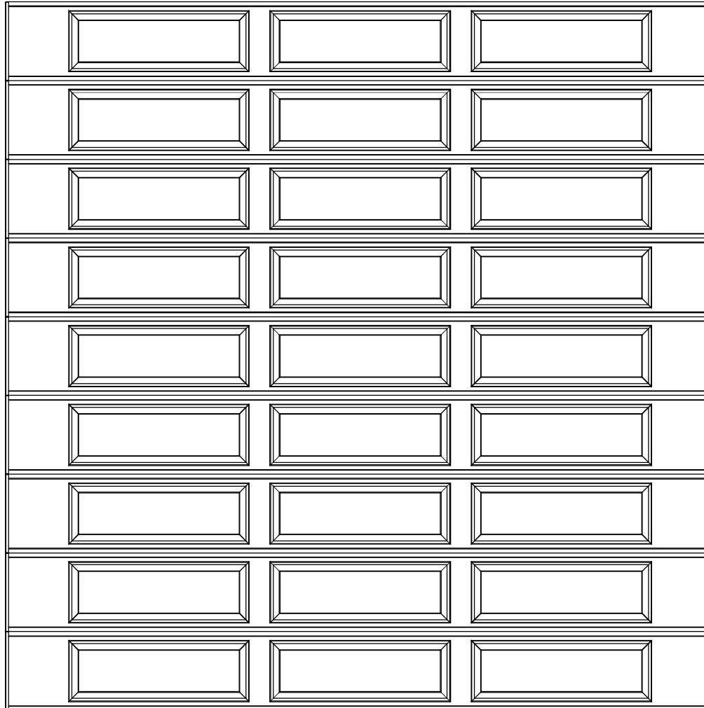
13'6" X 13'6" 8300/8500 ERP DESIGN 8 SECTION/ 3 PANEL SOLID TOP SECTION (9) 18" SECTIONS
