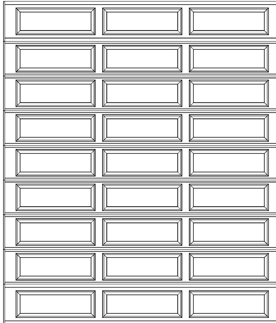
12'0" X 14'0" 8300/8500 ERP DESIGN 8 SECTION / 3 PANEL SOLID TOP SECTION (7) 18" & (2) 20.8" SECTIONS
