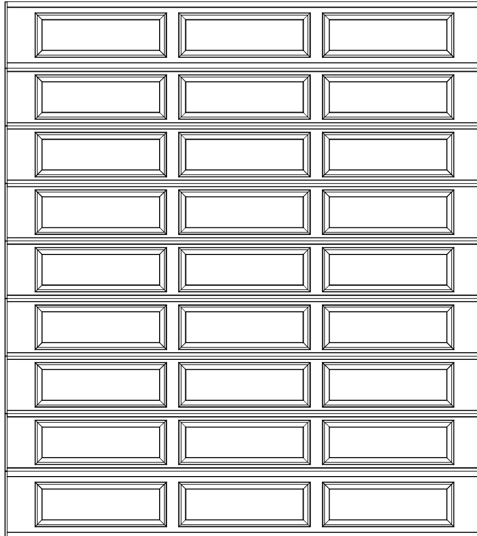
12'6" X 14'0" 8300/8500 ERP DESIGN 8 SECTION/ 3 PANEL SOLID TOP SECTION (7) 18" & (2) 20.8" SECTIONS
