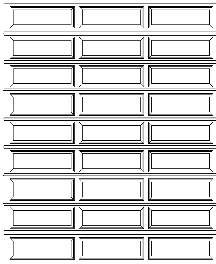
11'6" X 14'0" 8300/8500 ERP DESIGN 8 SECTION/ 3 PANEL SOLID TOP SECTION (7) 18" & (2) 20.8" SECTIONS
