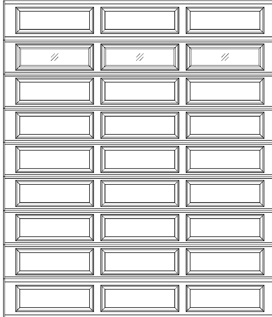
12'0" X 14'0" 8300/8500 ERP DESIGN 8 SECTION / 3 PANEL STYLELINE II INTERMEDIATE SECTION 8 SECTION SHOWN (7) 18" & (2) 20.8" SECTIONS
