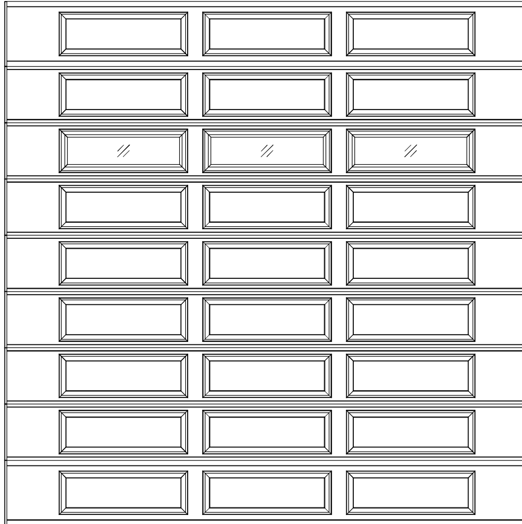
14'0" X 14'0" 8300/8500 ERP DESIGN 8 SECTION/ 3 PANEL STYLELINE II INTERMEDIATE 7 SECTION SHOWN (7) 18" & (2) 20.8" SECTIONS
