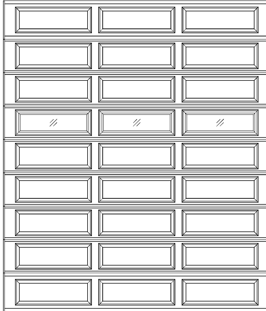
12'0" X 14'0" 8300/8500 ERP DESIGN 8 SECTION / 3 PANEL STYLELINE II INTERMEDIATE SECTION 6 SECTION SHOWN (7) 18" & (2) 20.8" SECTIONS
