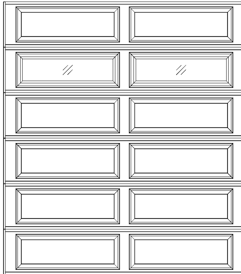
8'0" X 9'0" 8300/8500 ERP DESIGN 6 SECTION/ 2 PANEL STYLELINE II INTERMEDIATE 5 SECTION SHOWN (6) 18" SECTIONS
