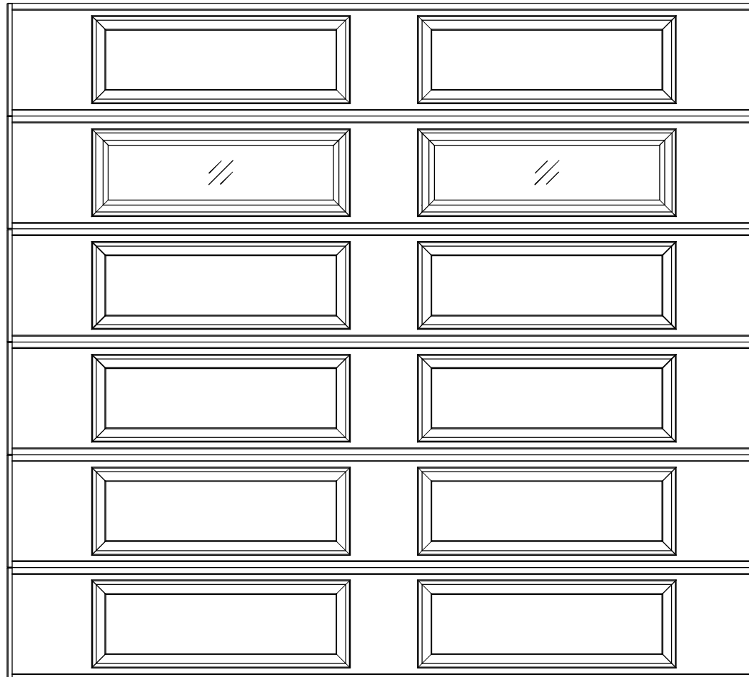
10'0" X 9'0" 8300/8500 ERP DESIGN 6 SECTION/ 2 PANEL STYLELINE II INTERMEDIATE 5 SECTION SHOWN (6) 18" SECTIONS
