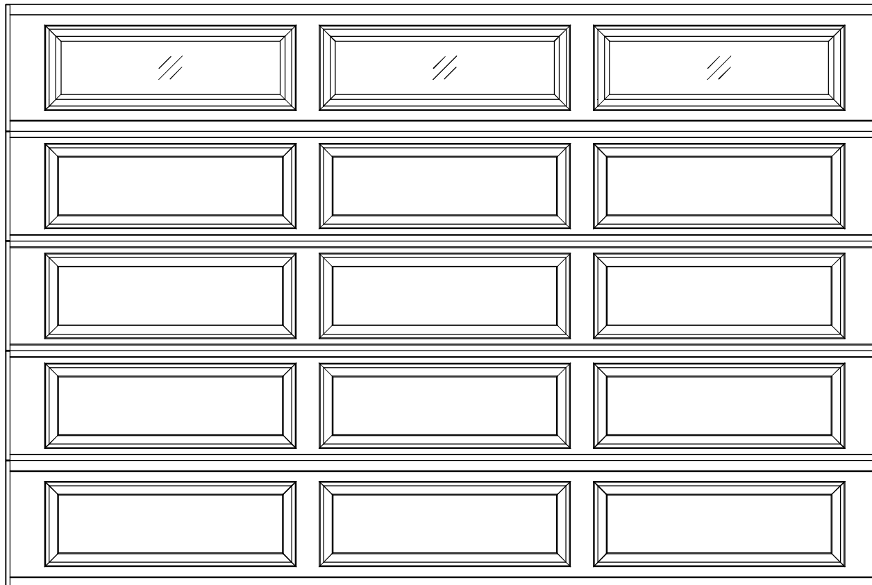
12'0" X 8'0" 8300/8500 ERP DESIGN 5 SECTION / 3 PANEL STYLELINE II TOP SECTION SHOWN (3) 18" & (2) 20.8" SECTIONS
