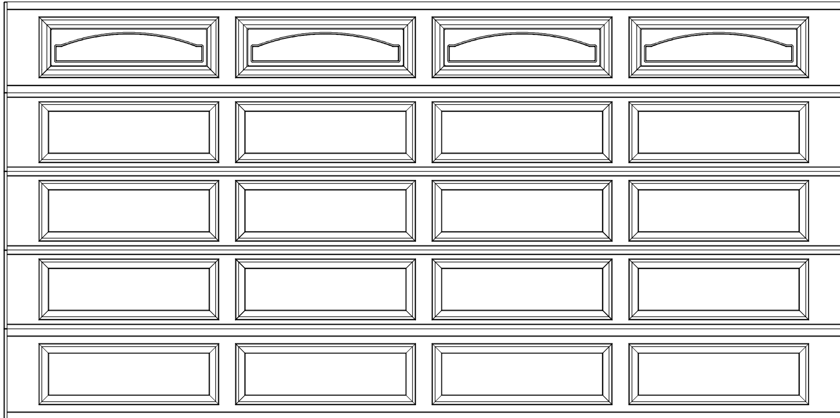
16'0" X 8'0" 8300/8500 ERP DESIGN 5 SECTION/ 4 PANEL CATHEDRAL II TOP SECTION SHOWN (3) 18" & (2) 20.8" SECTIONS
