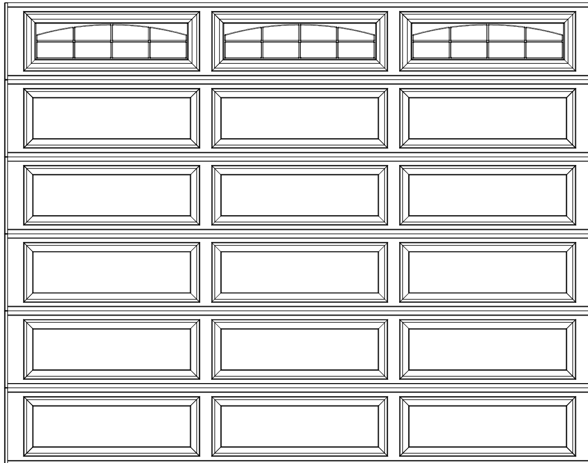
11'6" X 9'0" 8300/8500 ERP DESIGN 6 SECTION/ 3 PANEL CASCADE II TOP SECTION SHOWN (6) 18" SECTIONS
