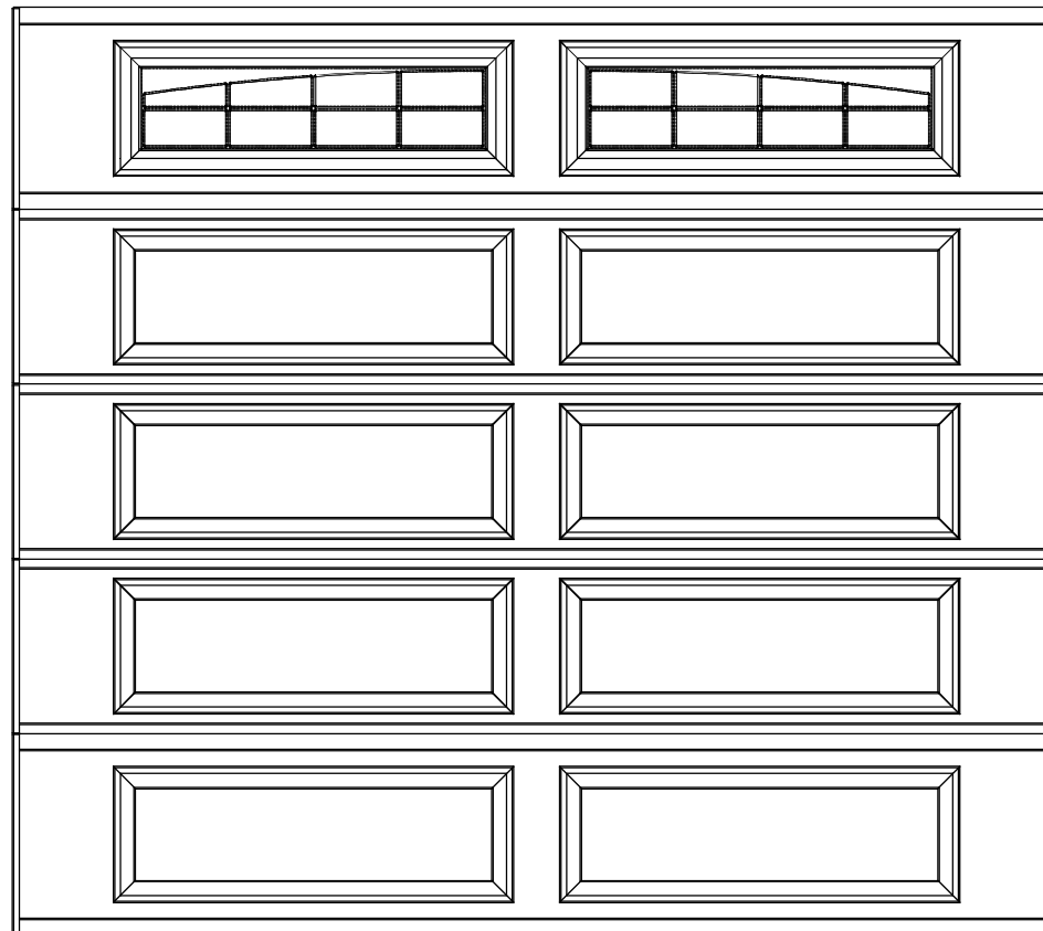
9'0" X 8'0" 8300/8500 ERP DESIGN 5 SECTION/ 2 PANEL ARCHED STOCKTON TOP SECTION SHOWN (3) 18" & (2) 20.8" SECTIONS
