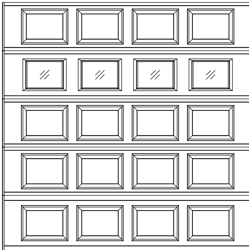
9'0" X 9'0" 8300/8500 CRP DESIGN 5 SECTION/4 PANEL STYLELINE I INT4 SECTION SHOWN (4) 20.8" & (1) 24" SECTIONS
