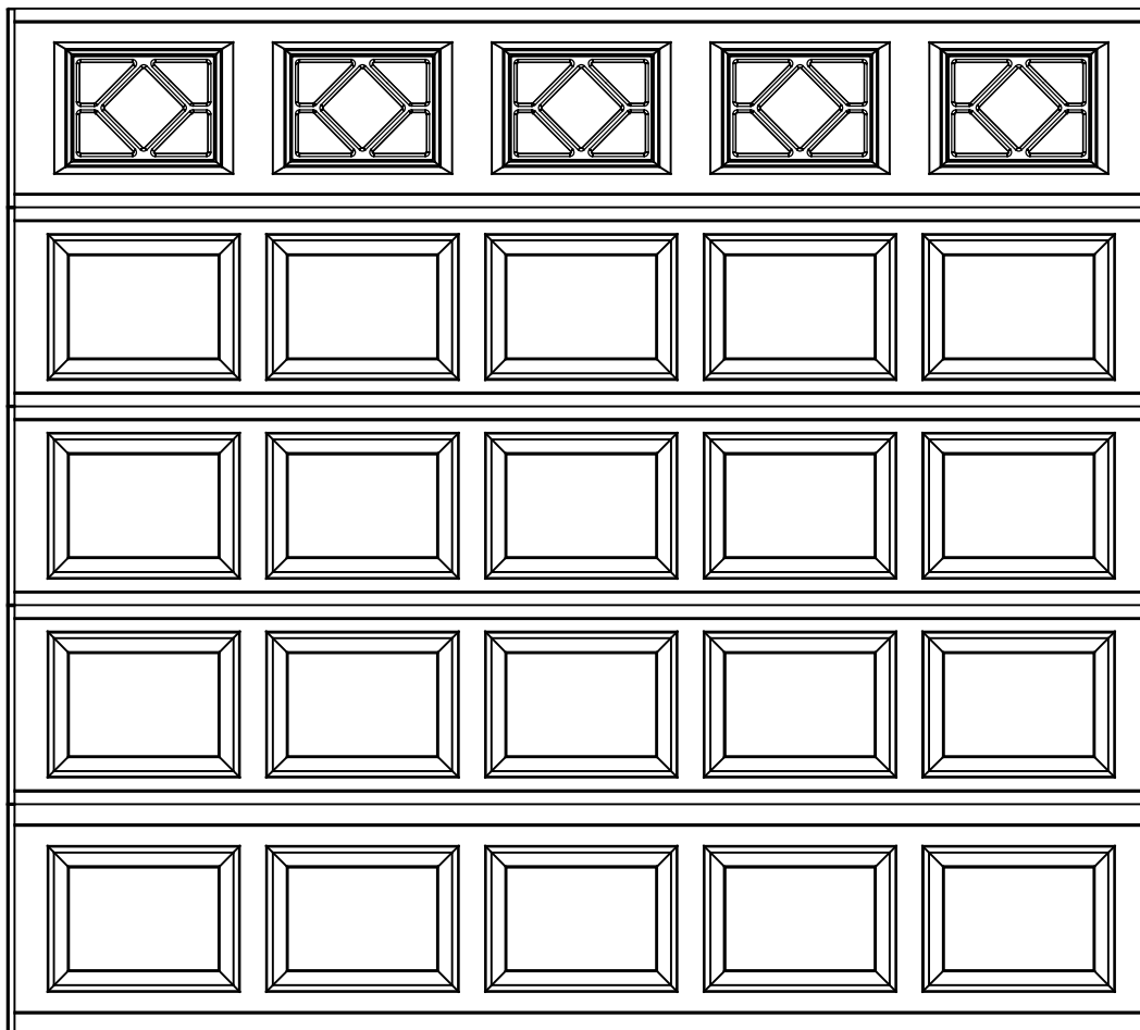
10'0" X 9'0" 8300/8500 CRP DESIGN 5 SECTION/5 PANEL WATERTON I TOP SECTION SHOWN (4) 20.8" SECTIONS & (1) 24" Section
