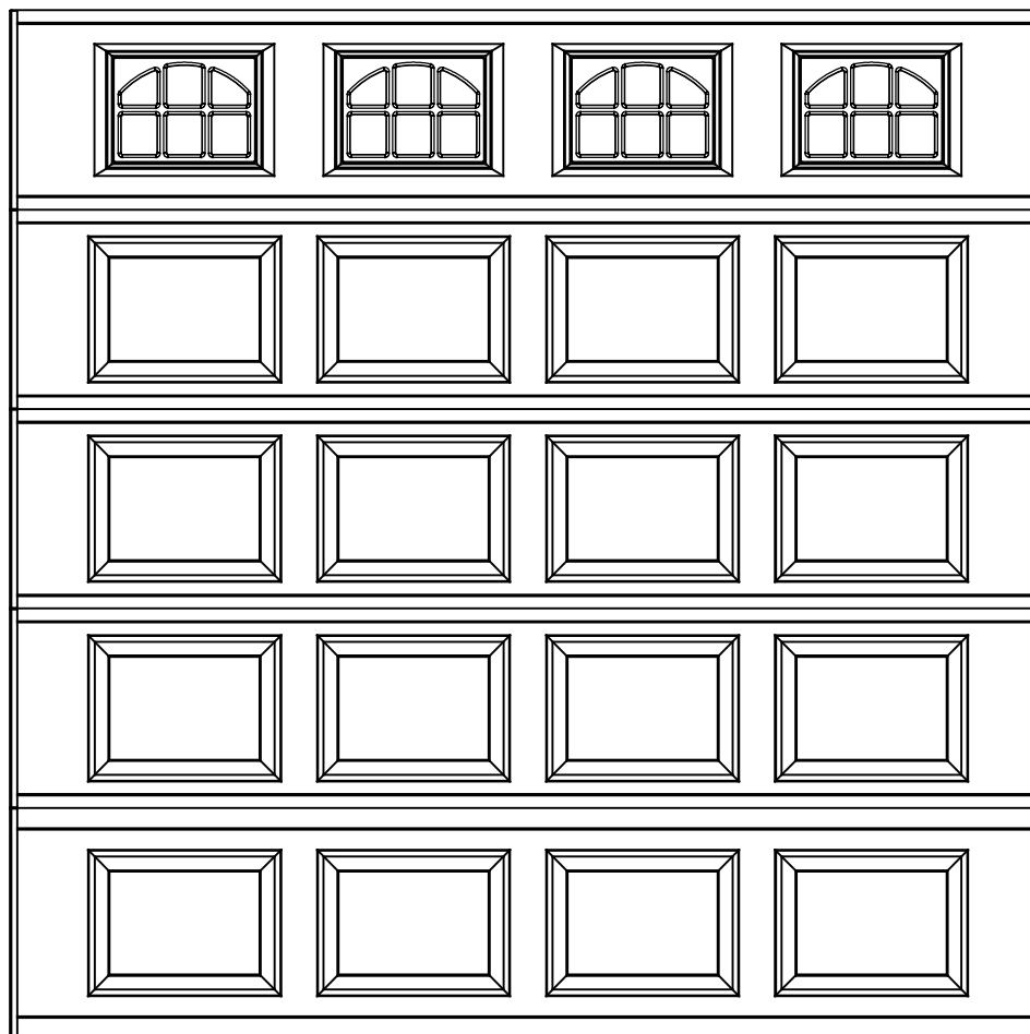
9'0" X 9'0" 8300/8500 CRP DESIGN 5 SECTION/4 PANEL CASCADE I TOP SECTION SHOWN (4) 20.8" & (1) 24" SECTIONS
