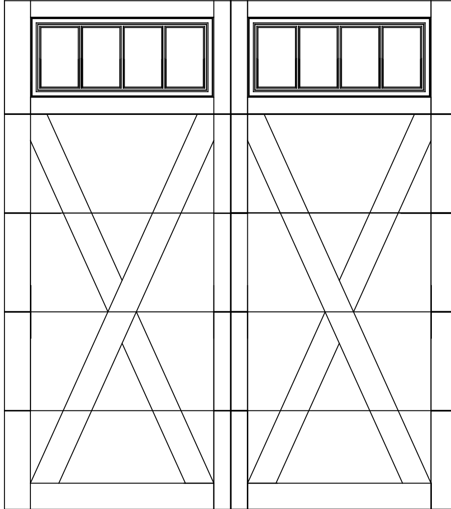
8x9 6600 LEXINGTON 5 SECTION/2 PANEL FRAMED STOCKBRIDGE TOP SECTION SHOWN CONSISTS OF (1) 24" & (4) 20.8" SECTIONS
