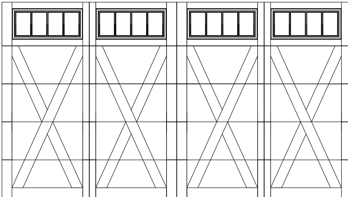
16x9 6600 LEXINGTON 5 SECTION/4 PANEL FRAMED STOCKBRIDGE TOP SECTION SHOWN CONSISTS OF (1) 24" & (4) 20.8" SECTIONS
