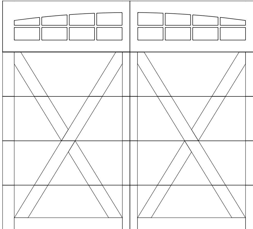
10'x9' 6600 LEXINGTON 5 SECTION/2 PANEL ROUTED SOMERTON TOP SECTION SHOWN CONSISTS OF (4) 20.8" & (1) 23.8" SECTIONS
