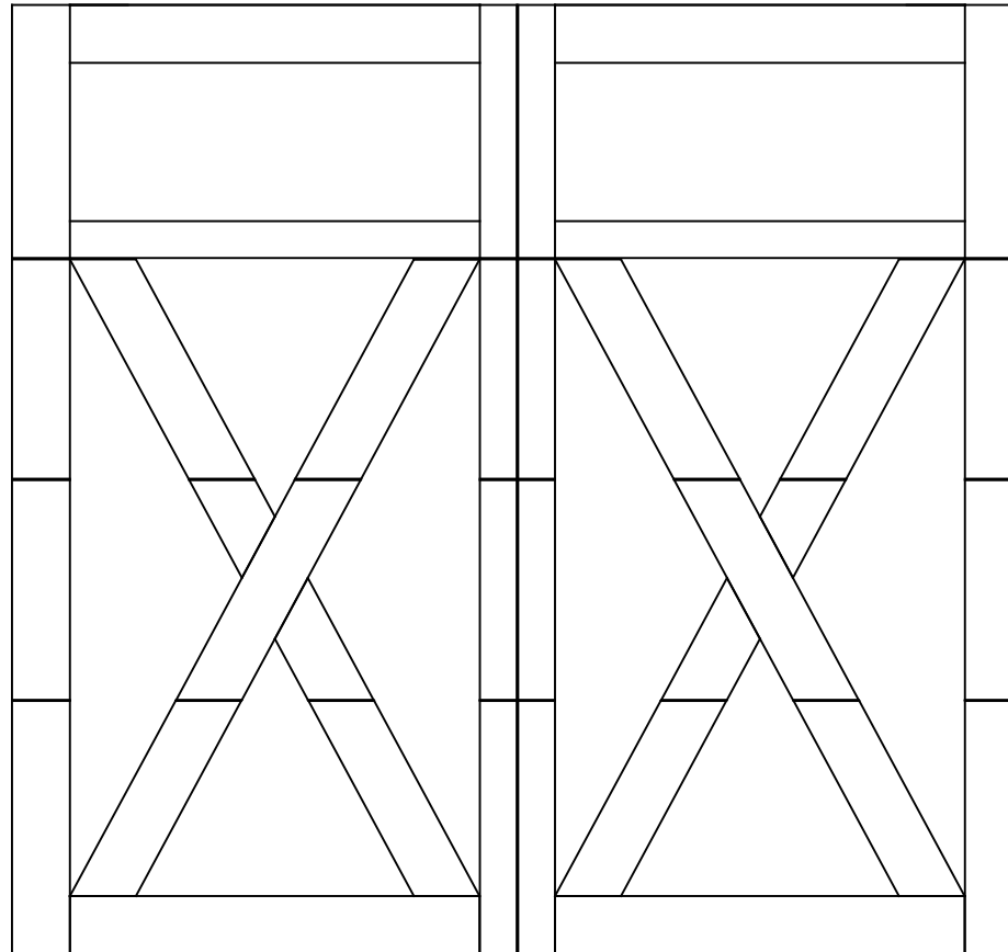
8'x7'6" 6600 LEXINGTON 4 SECTION/2 PANEL SOLID SQUARE TOP SECTION SHOWN CONSISTS OF (2) 20.8" & (2) 24.0 SECTIONS
