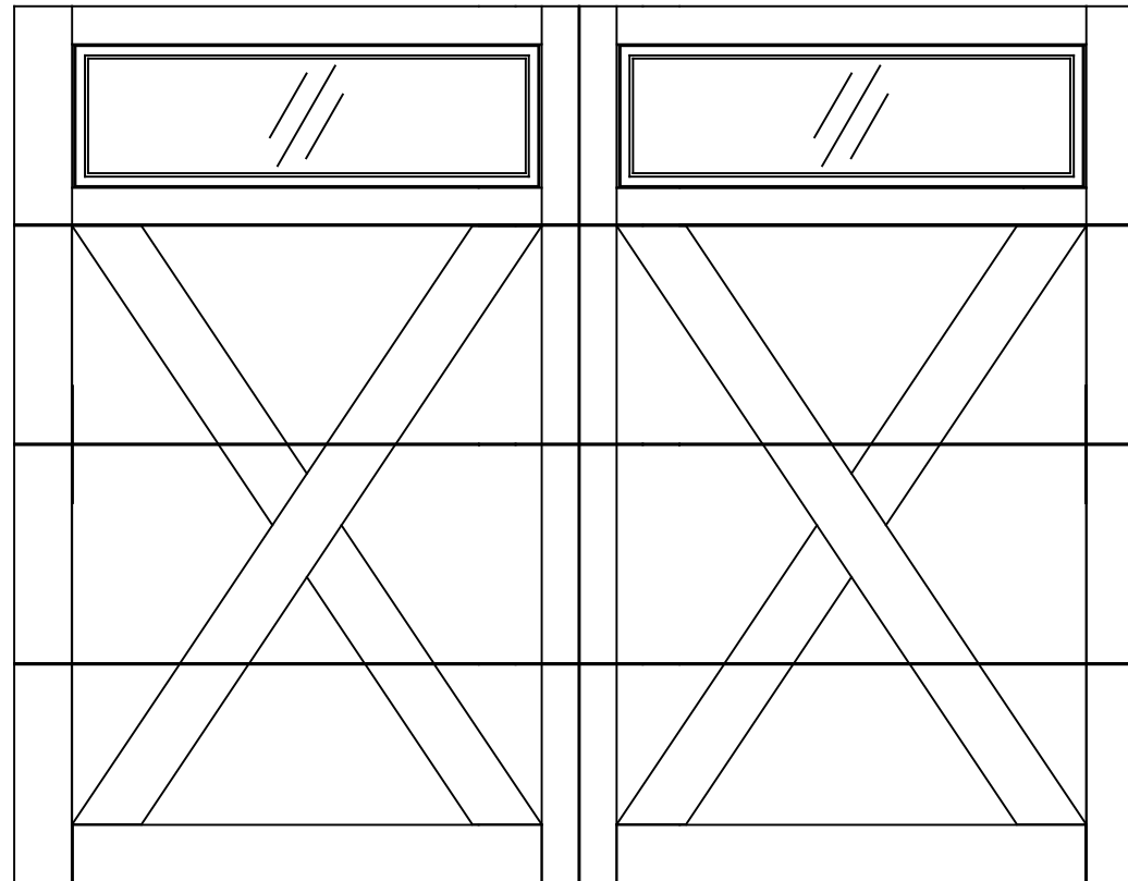
9x7 6600 LEXINGTON 4 SECTION/2 PANEL PLAIN GLAZED FRAMED TOP SECTION SHOWN CONSISTS OF (4) 20.8" SECTIONS
