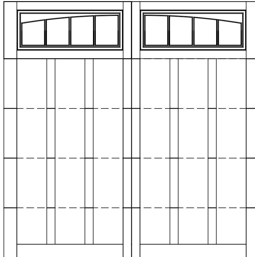
9x9 6600 BRUNSWICK 5 SECTION/2 PANEL FRAMED WYNDBRIDGE TOP SECTION SHOWN CONSISTS OF (4) 20.8" & (1) 24" SECTIONS
