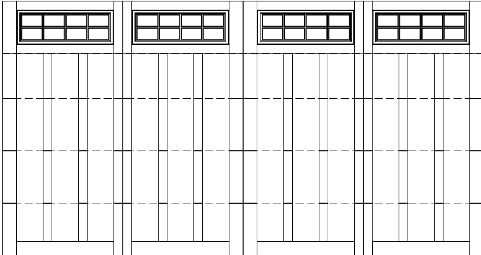
16'x8'6" 6600 BRUNSWICK 5 SECTION/4 PANEL FRAMED STOCKTON TOP SECTION SHOWN CONSISTS OF (4) 20.8" & (1) 18" SECTIONS
