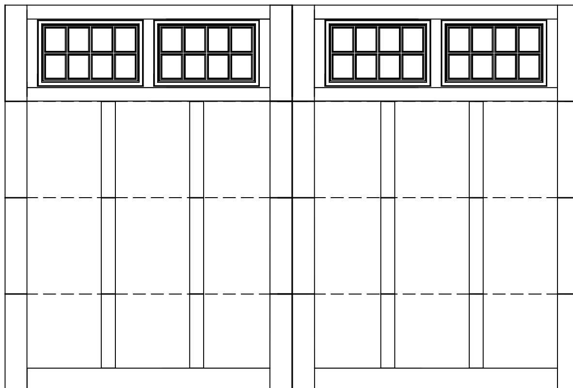
12x8 6600 BRUNSWICK 4 SECTION/2 PANEL FRAMED STOCKTON TOP SECTION SHOWN CONSISTS OF (4) 24.0" SECTIONS
