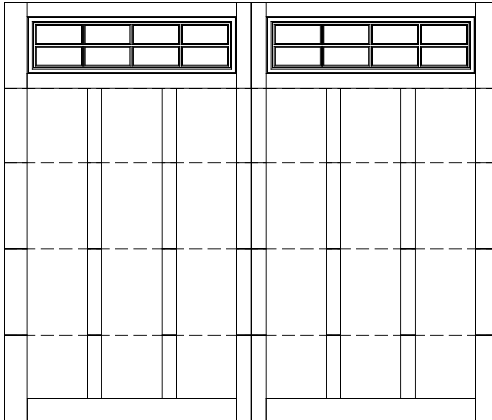
10'x8'6" 6600 BRUNSWICK 5 SECTION/2 PANEL FRAMED STOCKTON TOP SECTION SHOWN CONSISTS OF (4) 20.8" & (1) 18" SECTIONS
