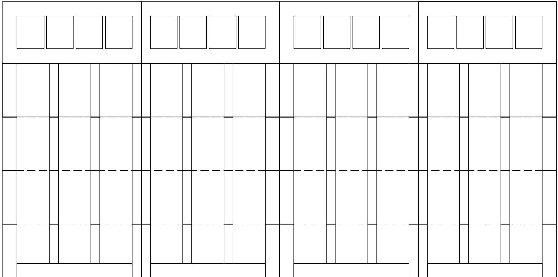
18x9 6600 BRUNSWICK 5 SECTION/4 PANEL ROUTED STOCKBRIDGE TOP SECTION SHOWN CONSISTS OF (4) 20.8" & (1) 24" SECTIONS
