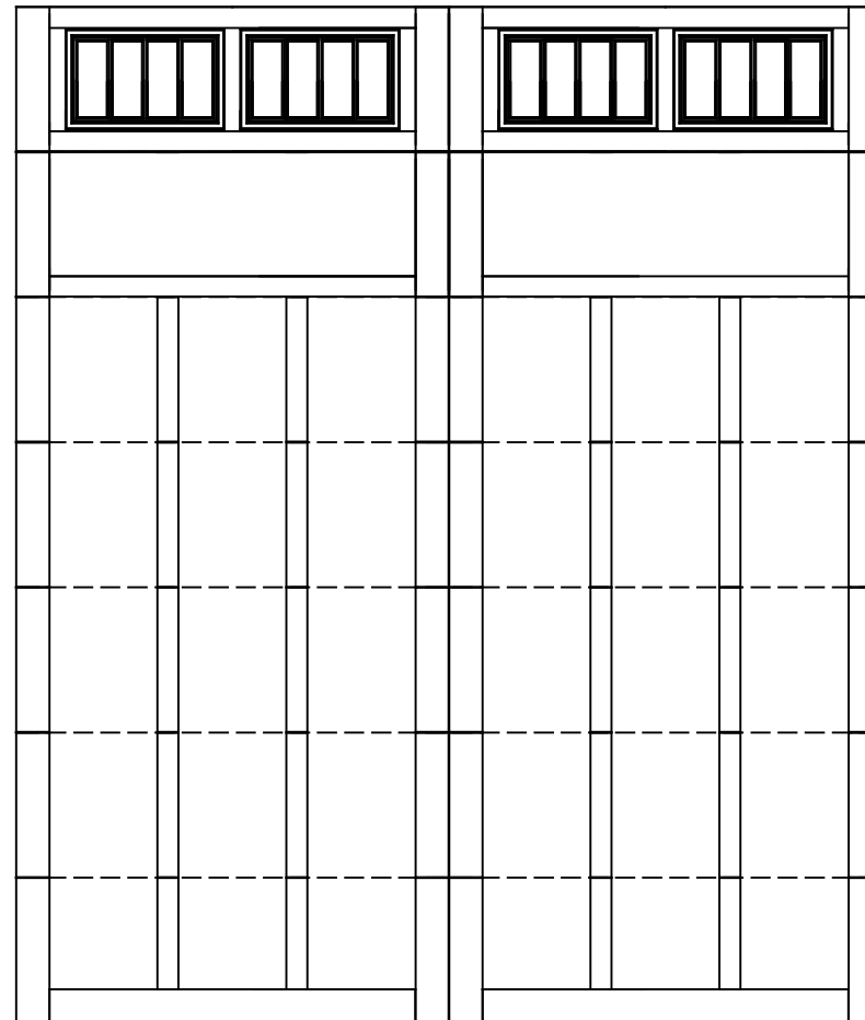
12x14 6600 BRUNSWICK 7 SECTION/2 PANEL FRAMED STOCKBRIDGE TOP SECTION SHOWN CONSISTS OF (7) 24.0" SECTIONS
