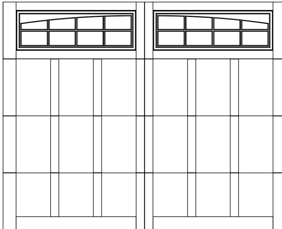
10x8 6600 BRUNSWICK 4 SECTION/2 PANEL FRAMED SOMERTON TOP SECTION SHOWN CONSISTS OF (4) 24.0" SECTIONS
