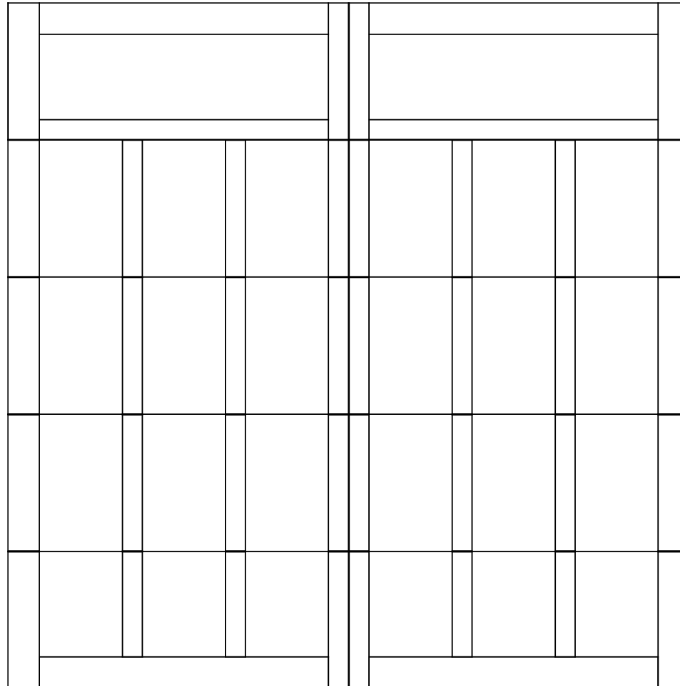
10x10 6600 BRUNSWICK 5 SECTION/2 PANEL SOLID SQUARE TOP SECTION SHOWN CONSISTS OF (5) 24.0" SECTIONS
