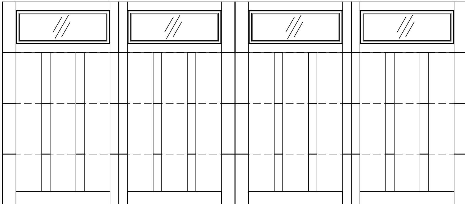
16x7 6600 BRUNSWICK 4 SECTION/4 PANEL PLAIN GLAZED FRAMED TOP SECTION SHOWN CONSISTS OF (4) 20.8" SECTIONS
