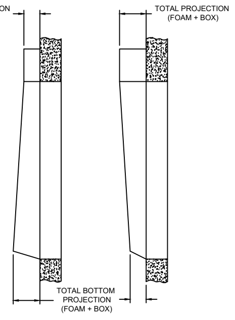
SECTION B-B TAPERED UP
