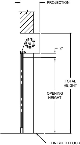
SECTION B-B
