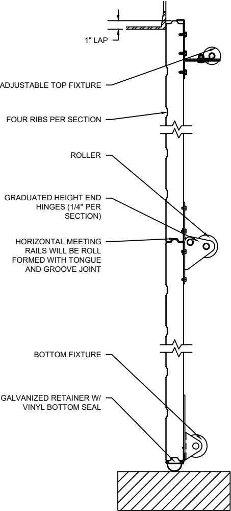
SECTION B-B
