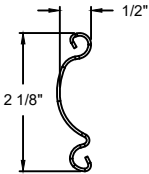
#2 SLAT SECTION
