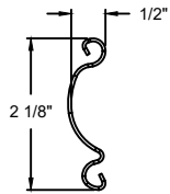
#2 SLAT SECTION
