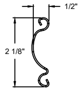
#2 SLAT SECTION
