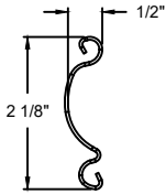
#2 SLAT SECTION
