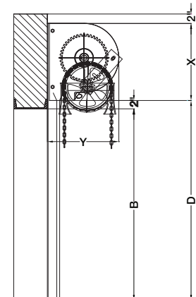
SECTION (FACE MOUNT)
