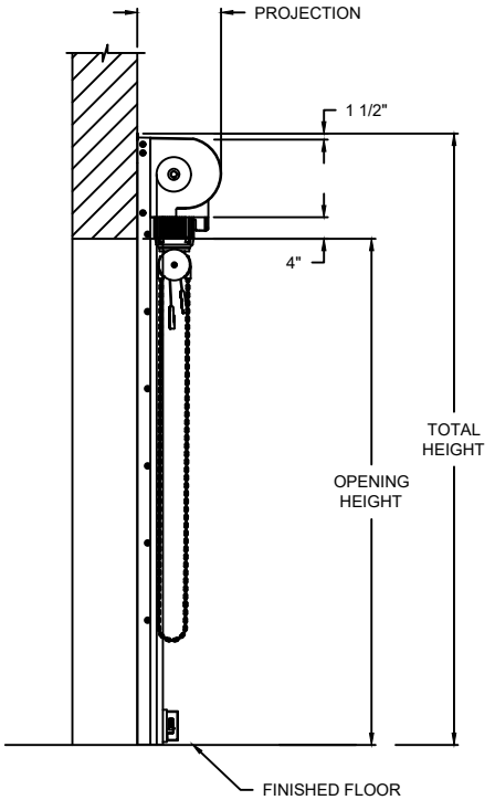
SECTION B-B
