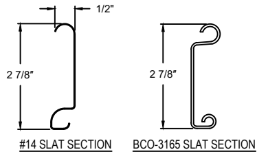
#14 SLAT SECTION
