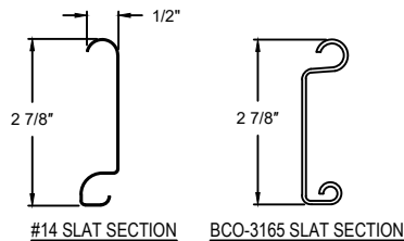
#14 SLAT SECTION BCO-3165 SLAT SECTION
