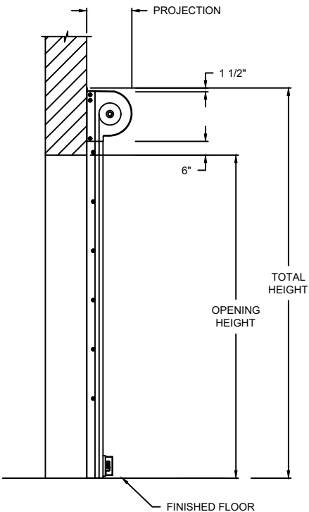
SECTION B-B
