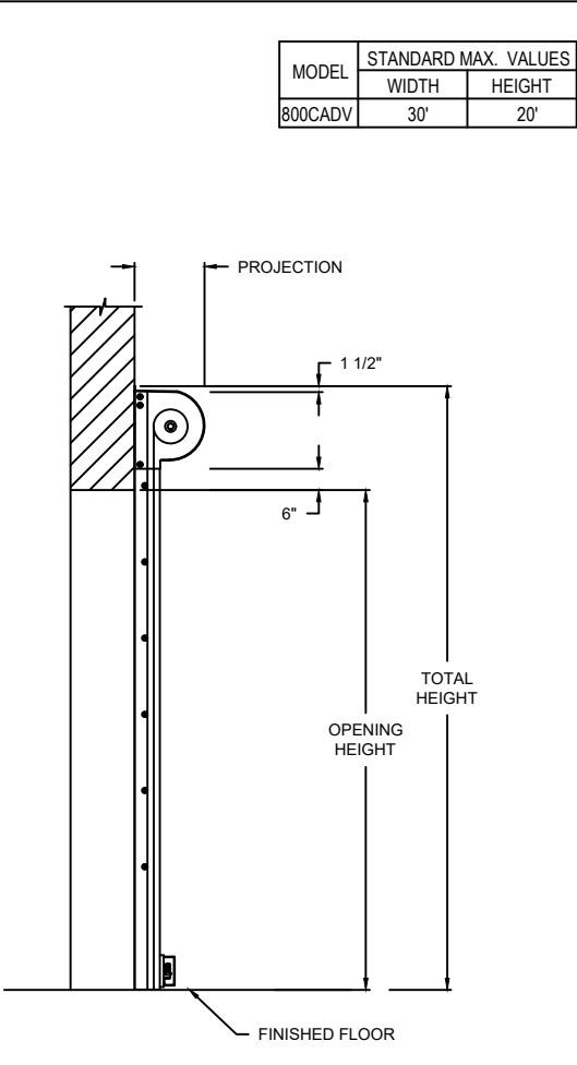
SECTION B-B
