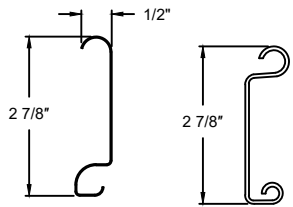
#14 SLAT DETAIL
