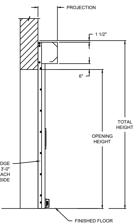
SECTION B-B
