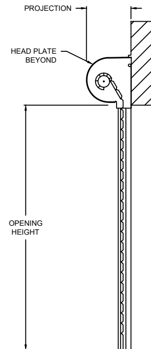
SECTION B-B
