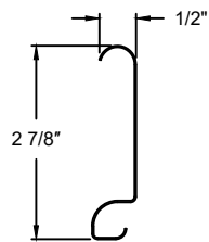
#14 SLAT SECTION
