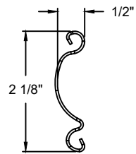
#2 SLAT SECTION
