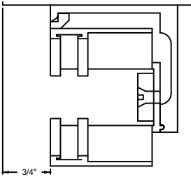
GUIDE DETAIL
